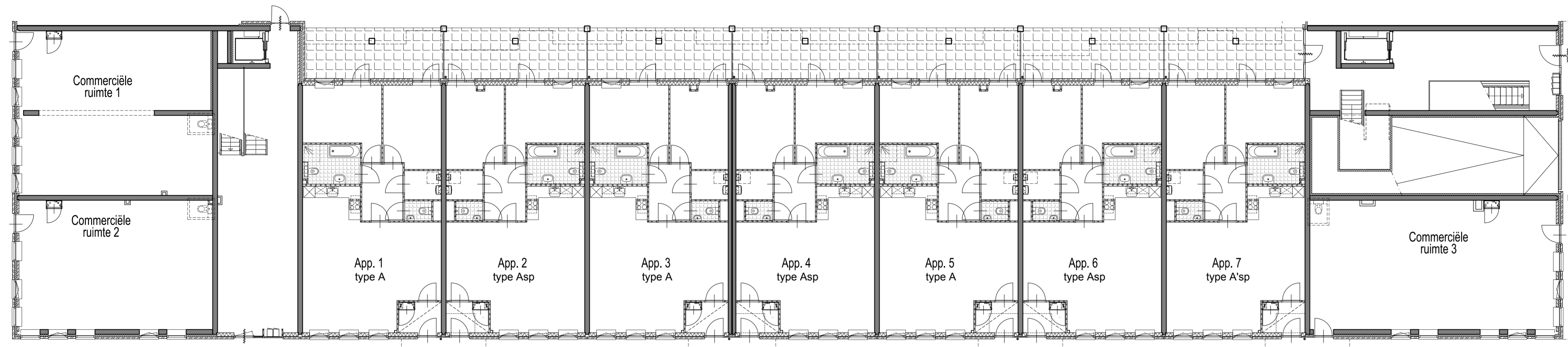
Begane grond (1:200)
